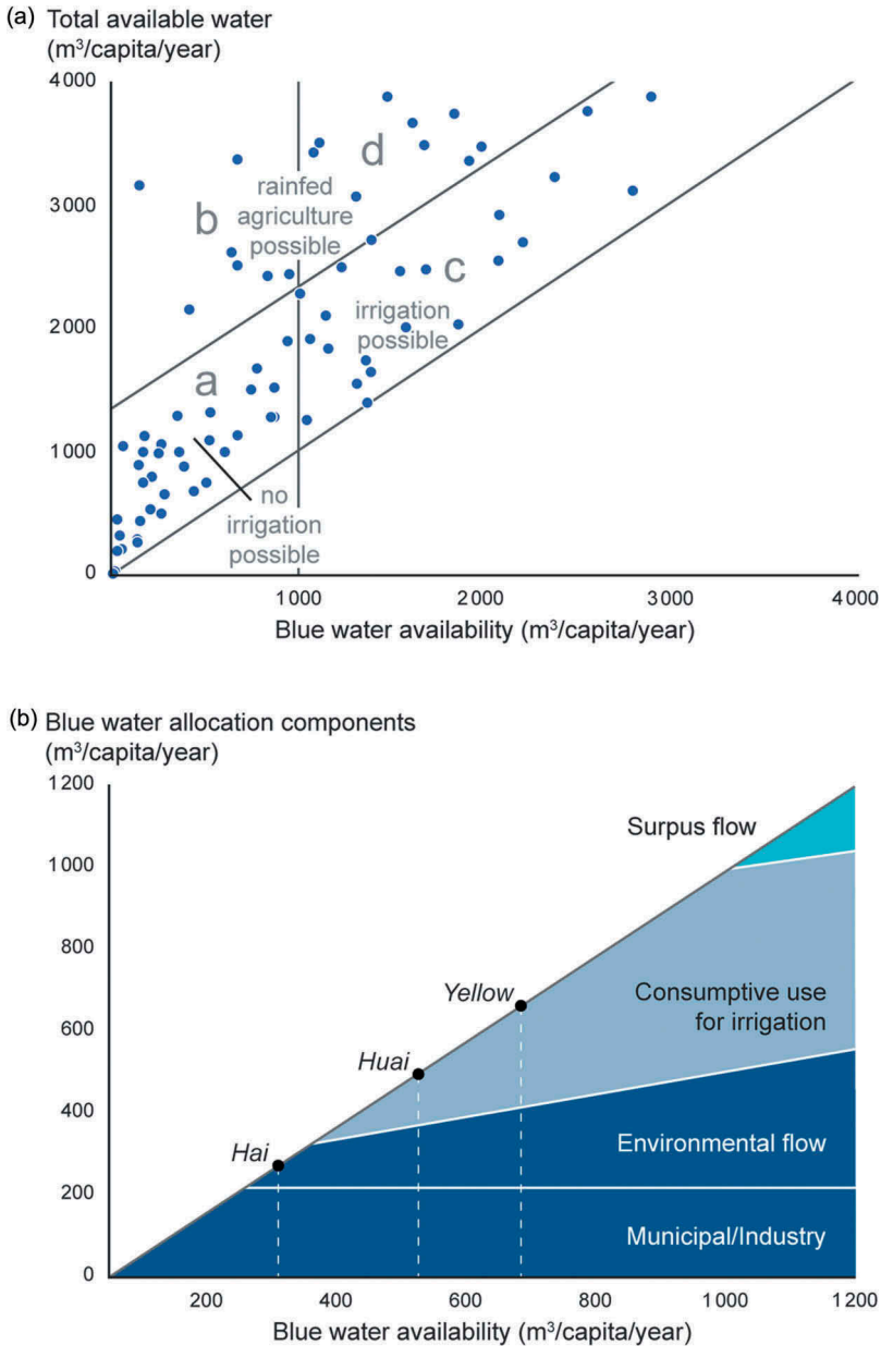
Figure 8. Food security and water supply. (a) Water availability constrains food security options. Enough green water for self-sufficient rainfed agriculture is available above the upper sloping line (areas b and d ). Enough blue water for irrigation exists beyond the vertical line (area c ). Inside area a , both green and blue water shortage implies dependence on food imports (adapted from Rockström, Karlberg, & Falkenmark, 2011). (b) Theoretically available water supply options, assuming 200 m 3 per person per year for municipal/industrial use, using the three Chinese rivers Hai, Huai, and Yellow (based on Falkenmark and Xia, 2012).
